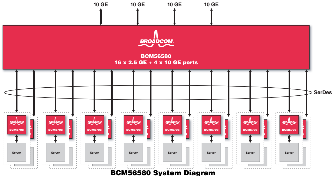
BCM56580 System Diagram
